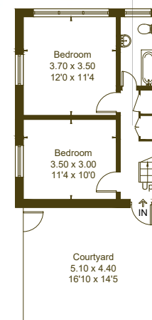
Cottage - Ground Floor
